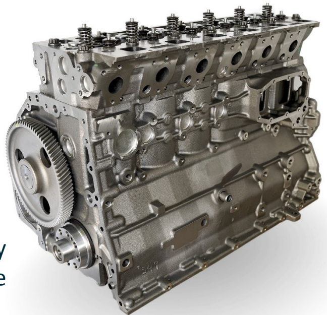
OE Germany R6 shortblock with cylinder head
